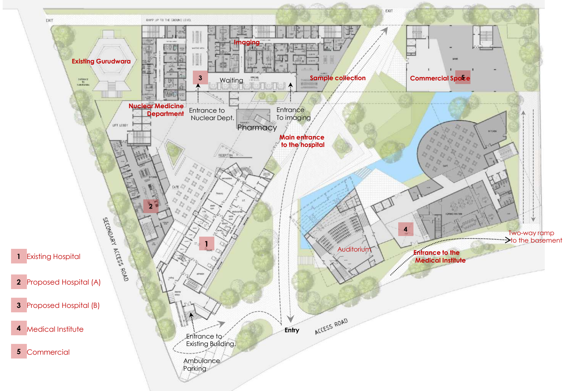
Ground Floor Plan(+1.80M)
