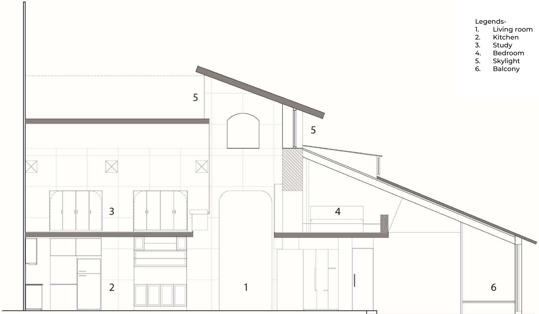
Sectional elevation B-B
