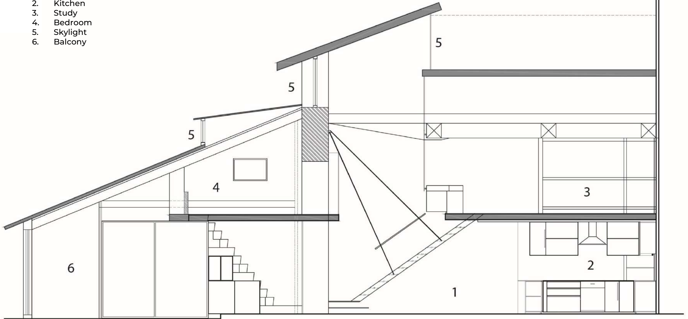
Sectional elevation A-A
